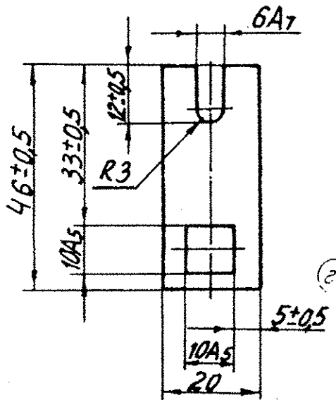
DEVELOPED VIEW
