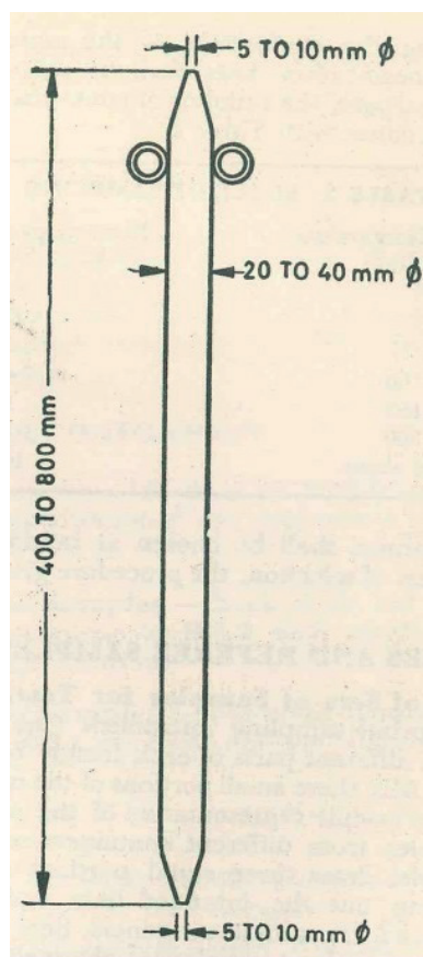
FIG. 4 SAMPLING TUBE
