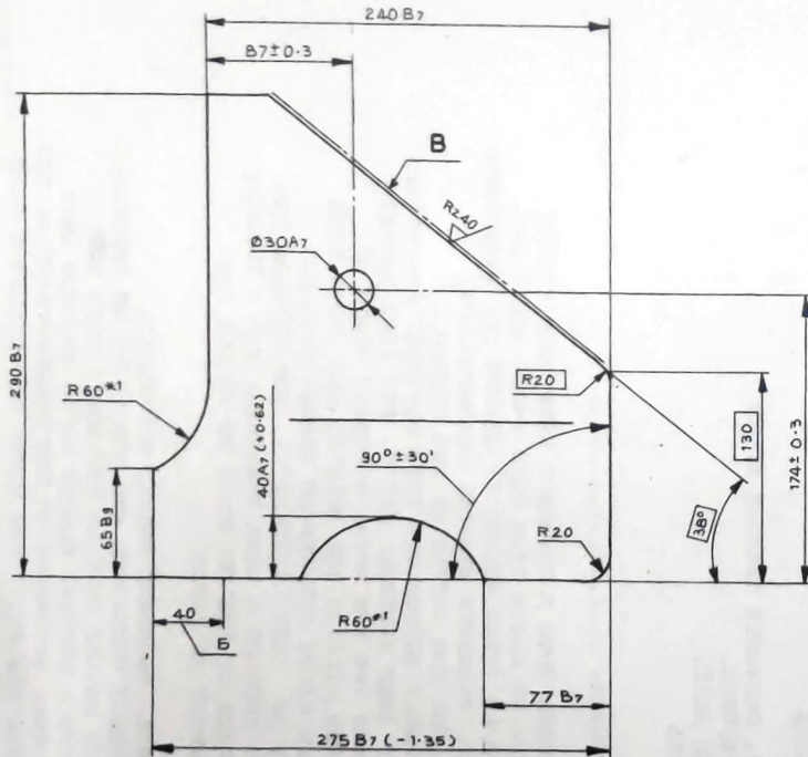
A-A SCALE TO: 1
