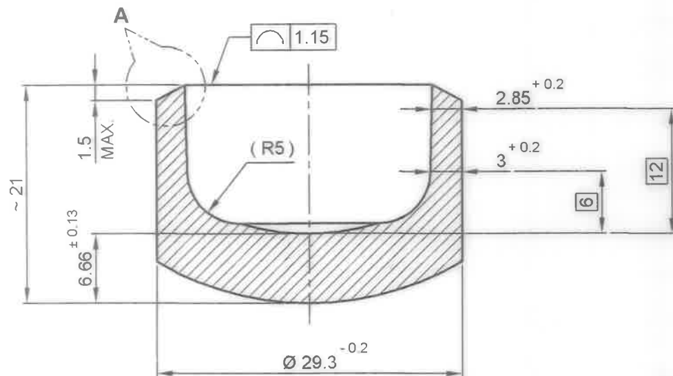
A ALTERNATIVE LIP
