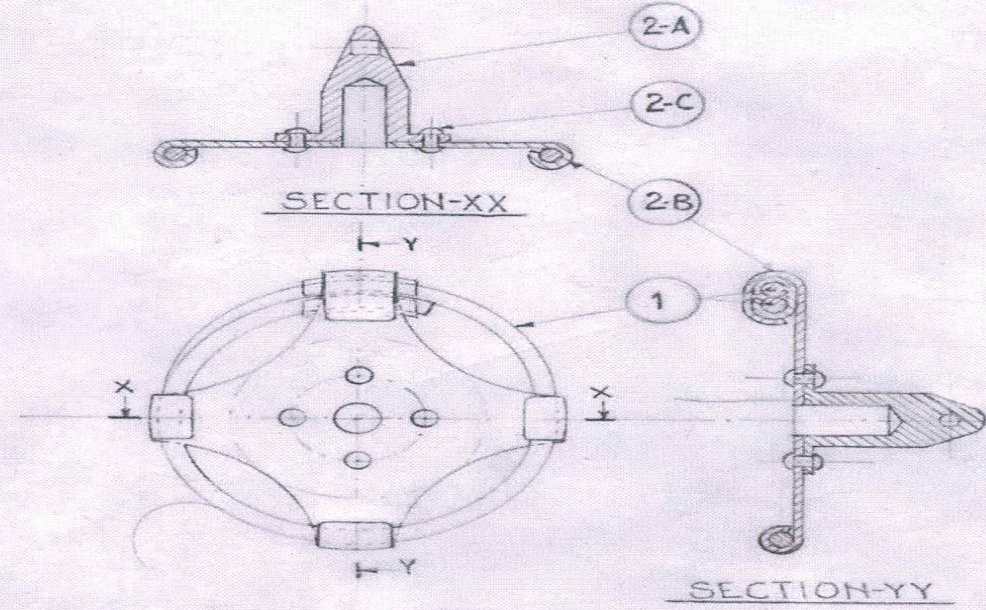
CONE SUB-ASSEMBLY 1-OFF
