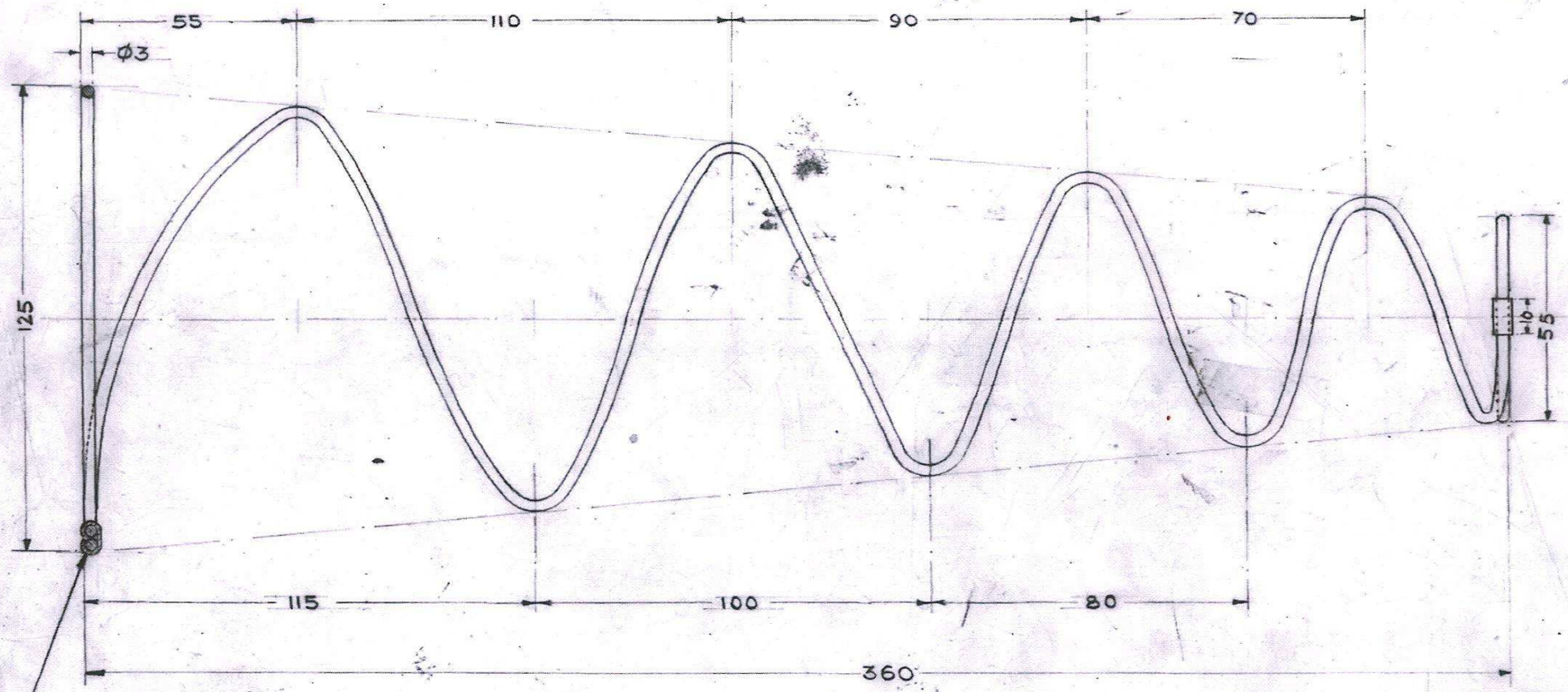
COIL SPRING SUBASSEMBLY 1-OFF
