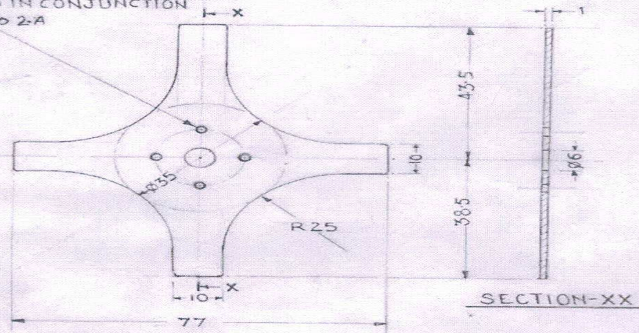
BASE PLATE 1-OFF
