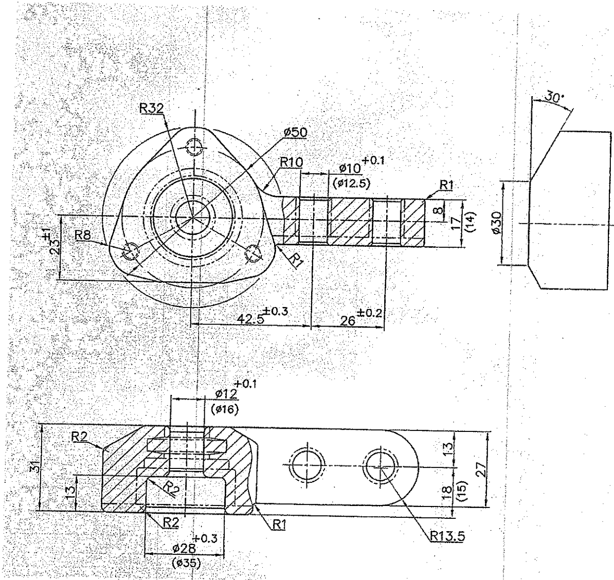
FIG: SUPPORT TO DRG. NO 172.61.025-1/C
