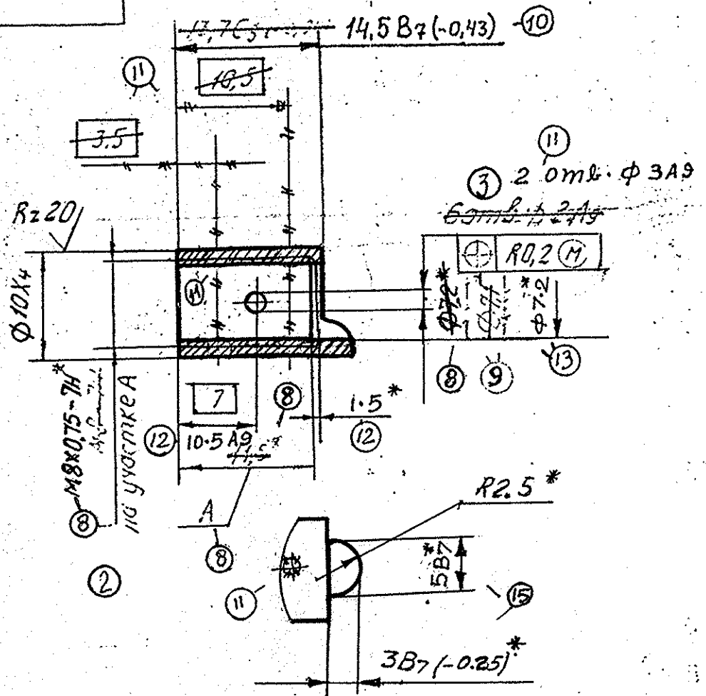
BUSHING
