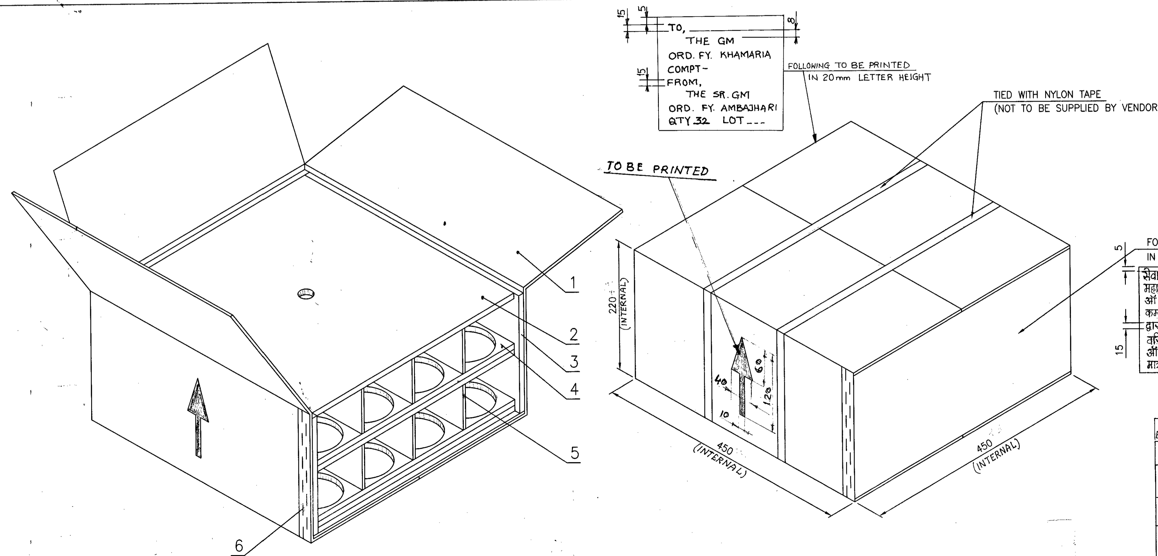
BOX IN CLOSED CONDITION.
