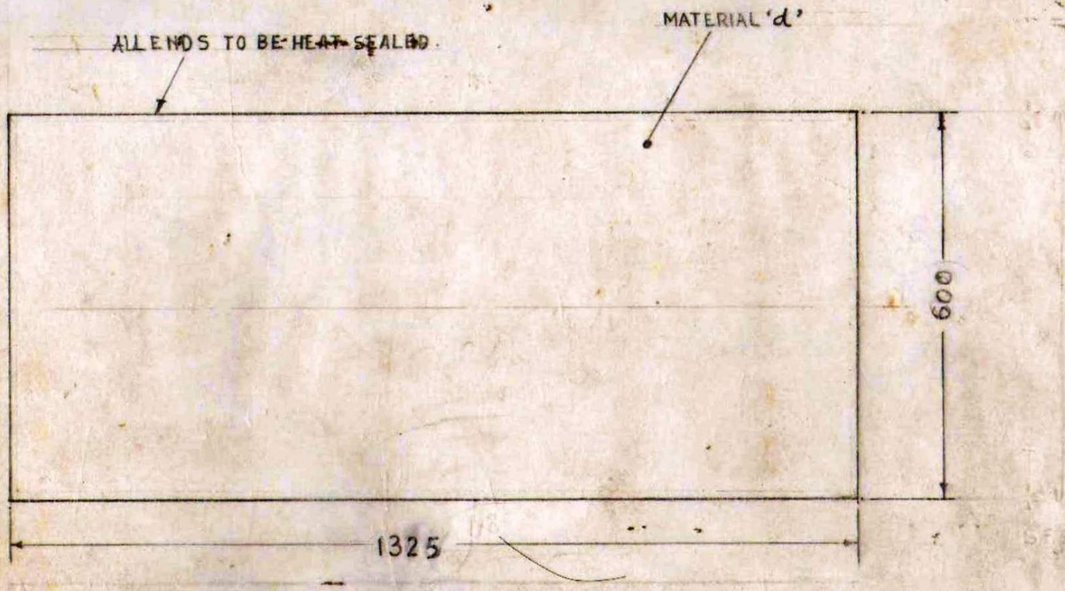
SIDE-CUM-BASE PIECE, DEVELOPMENT 1 - OFF
