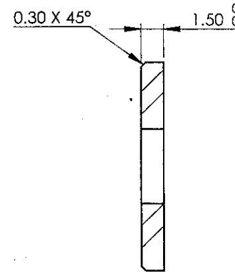
SECTION F-F
