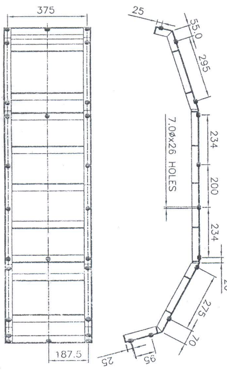
DETAILS DIMENSIONS OF HOLES FOR FITMENT OF RUBBER SHEET
