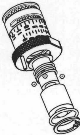
Exploded view
