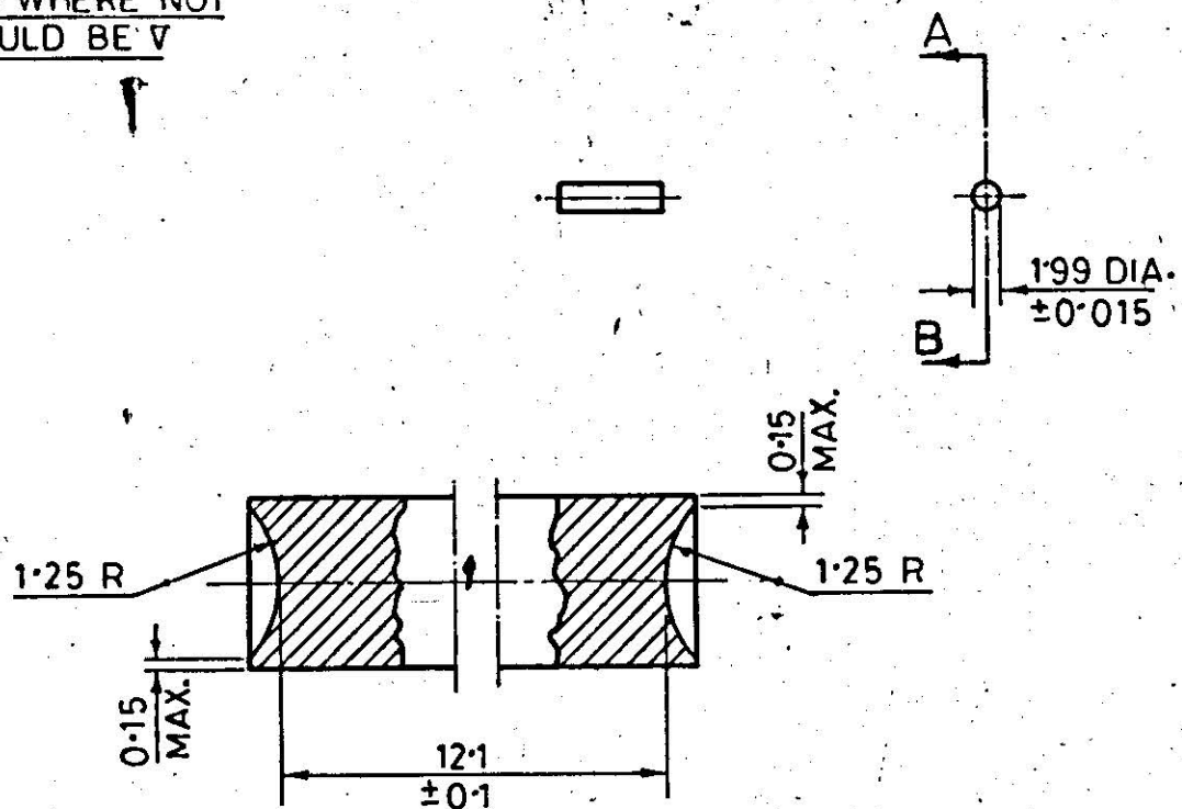
PARTIAL SECTION-A B
