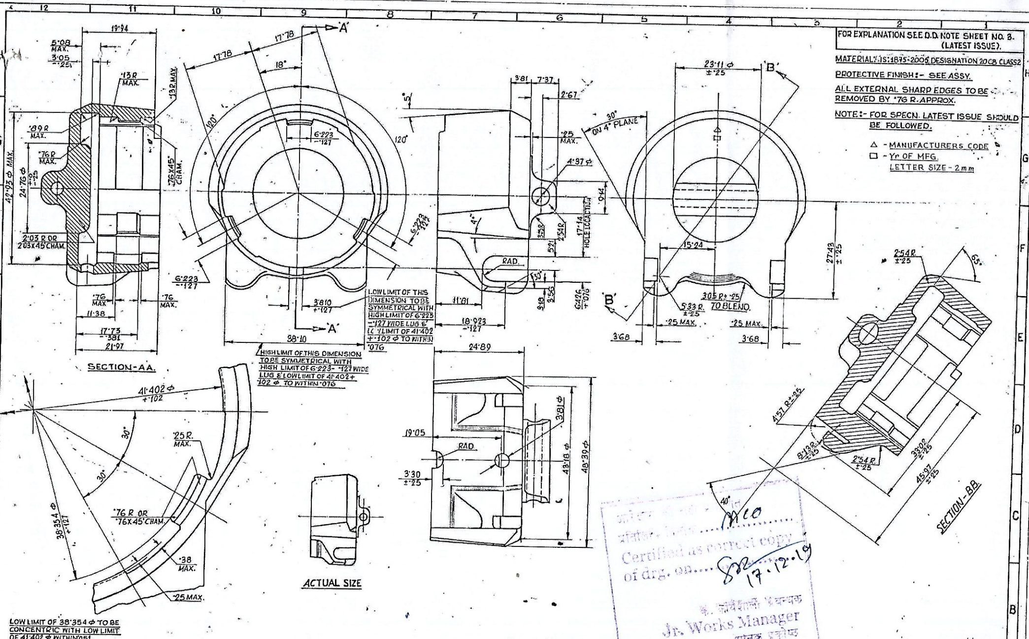
ENLARGED VIEW OF LUG FORM. SCALE - 5:1
