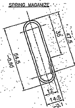
VIEW OF END COIL
