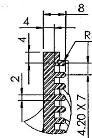
DETAIL E
