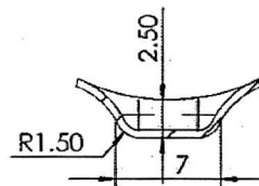
DETAIL E
