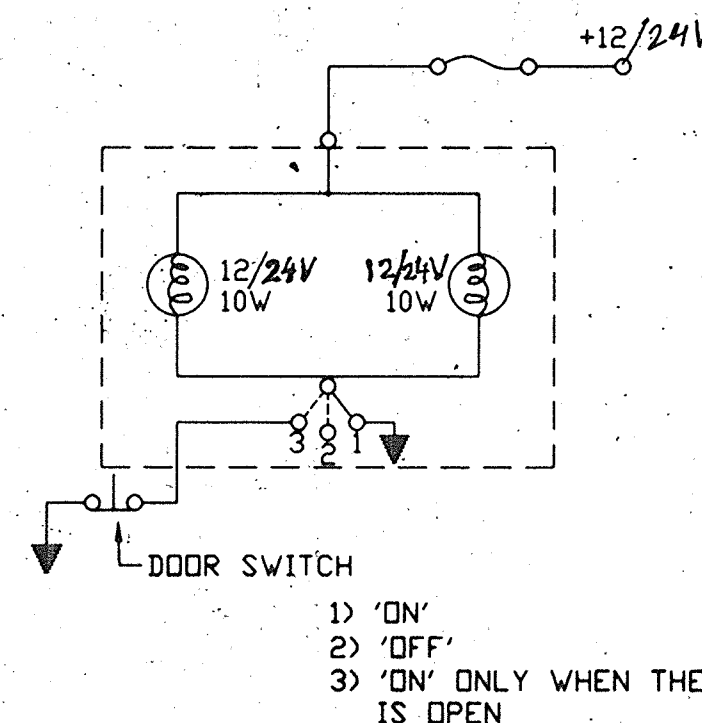
CIRCUIT DIAGRAM-A
