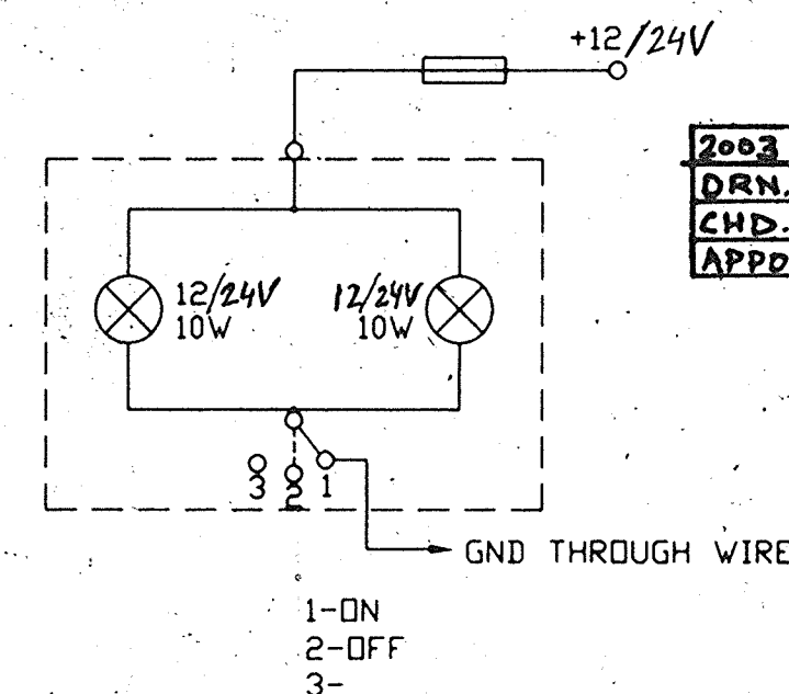
CIRCUIT DIAGRAM-BIPOLAR WIRING-B
