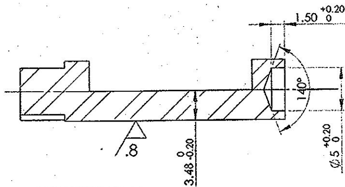
SECTION M-M
