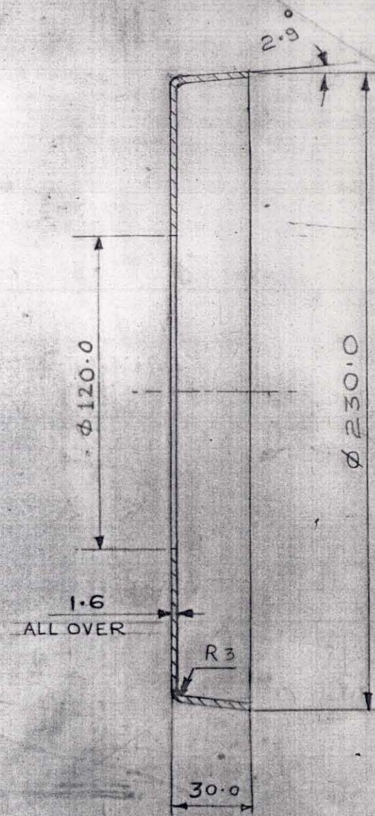
SECTION 'A-A'
