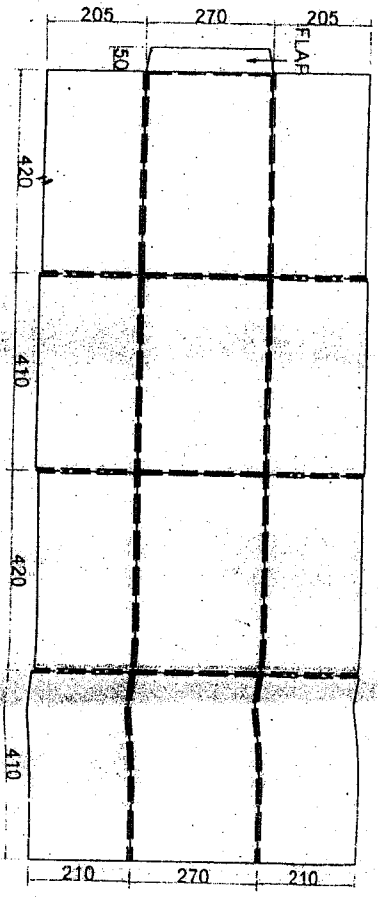
"BOX LAID FLAT SINGLE PIECE"
