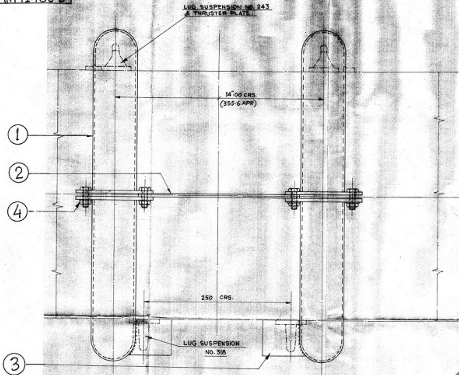
GENERAL ARRANGEMENT
