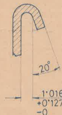
ENLARGED PART SECTION 'A A'
