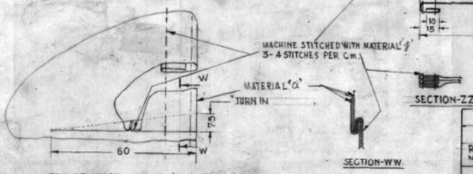
ENLARGEMENT AT 'P' SCALE:- 1:1
