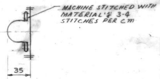
SECTION - YY
