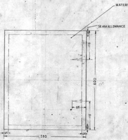
DEVELOPMENT SCALE:- 1:5
