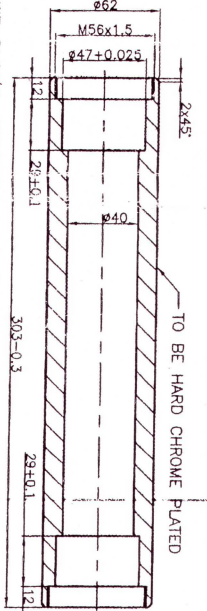
ROLLER SHEET NO.1
