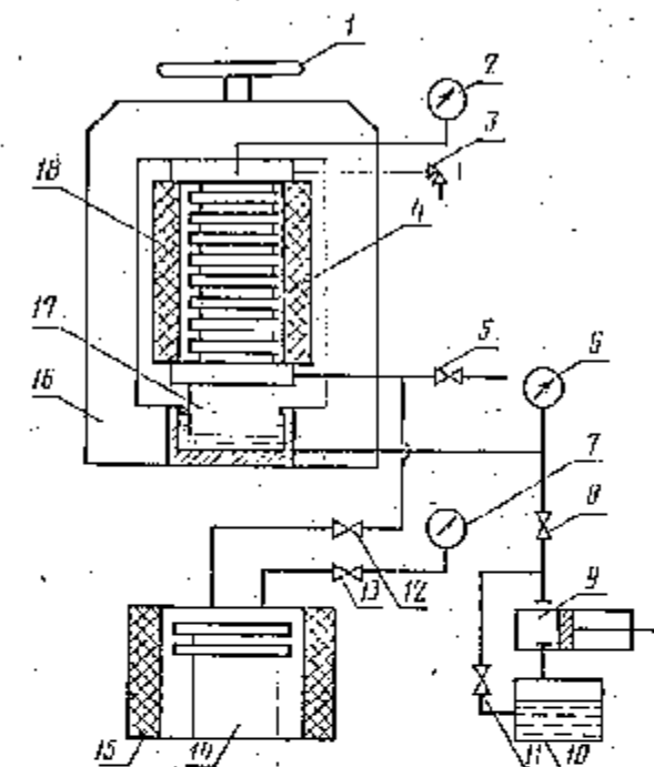
Ср. 12 GOST 481-80 SCHEMATIC OF AUTOCLAVE AP-1
