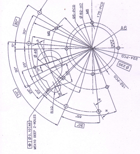
DETAIL-A6
