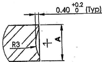
DETAIL D
