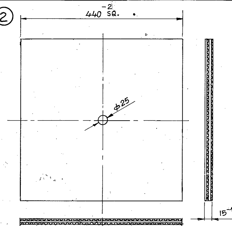
SHOCK ABSORBER (TOP & BOTTOM) NO. OFF - 2
