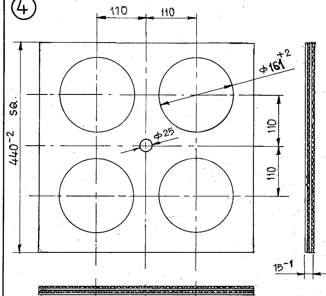
BASE SUPPORT NO. OFF - 1
