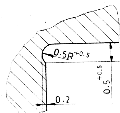
DETAIL - X SCALE - 10:1
