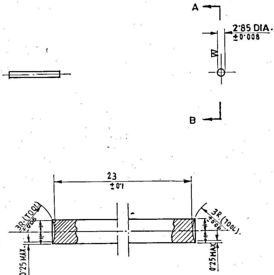
PARTIAL SECTION-AB SCALE:- 4:1
