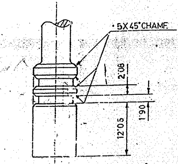
ENLARGED VIEW OF GROOVES SCALE: 2:1
