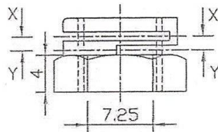
SECTION - XX
