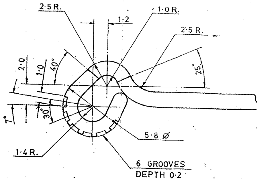
ENLARGED VIEW FROM -'A' SCALE - 5:1
