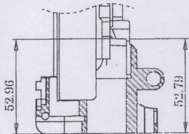
SECTION X-X
