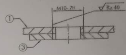
SECTION 'B-B' (enlarge view)
