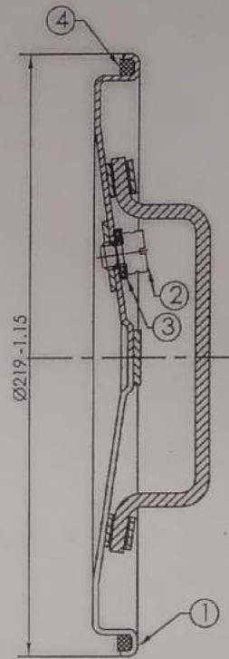
SECTION 'A-A'
