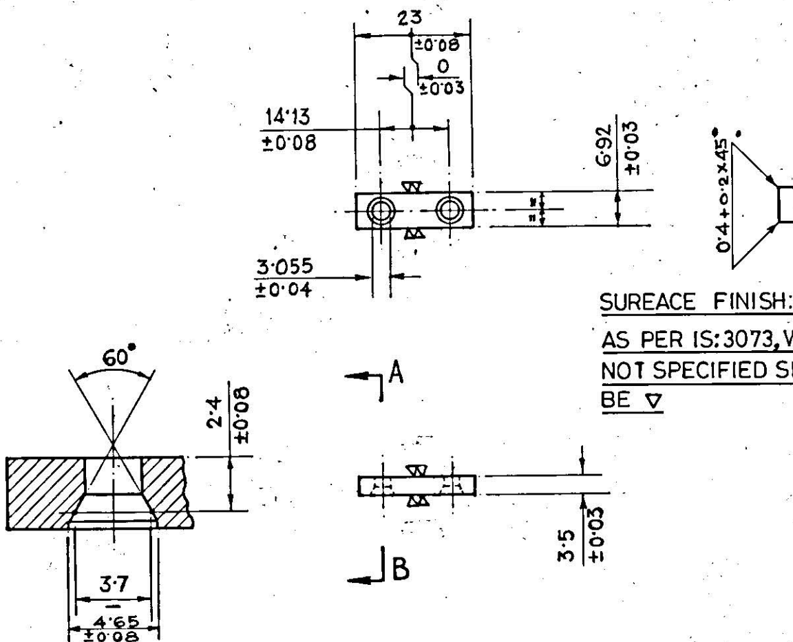
SECTION-AB SCALE ~ 4:1
