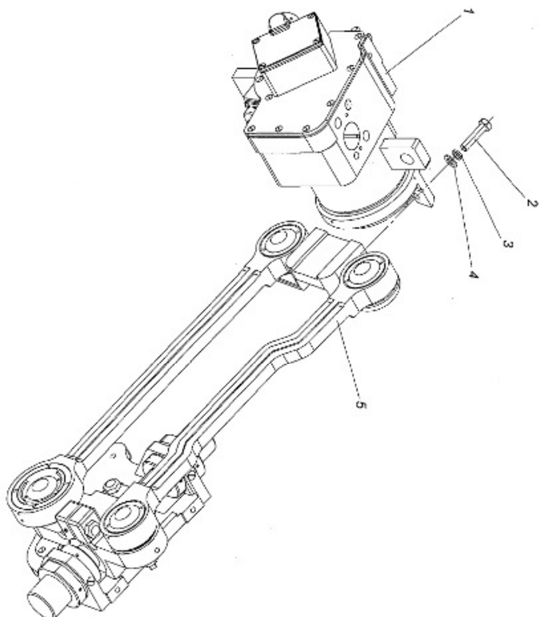
Figure 133. Position transducer 5172.320.040
