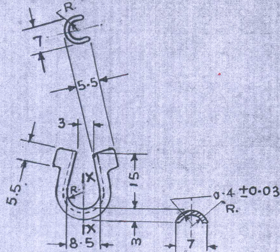
SECTION XX
