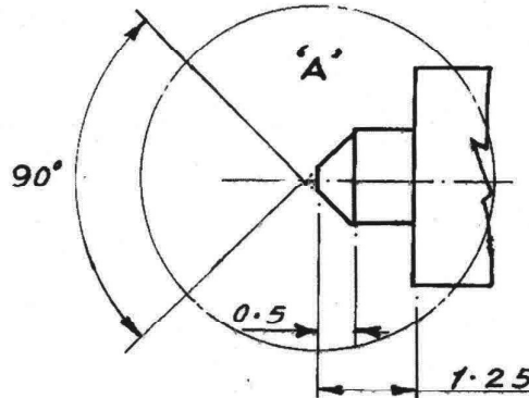
ENLARGED VIEW AT 'A' SCALE: 10:1
