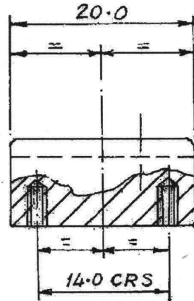
PART SECTION AT 'B-B'
