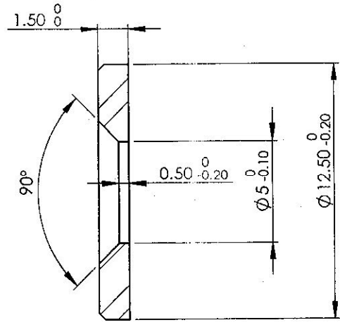
SECTION-EE
