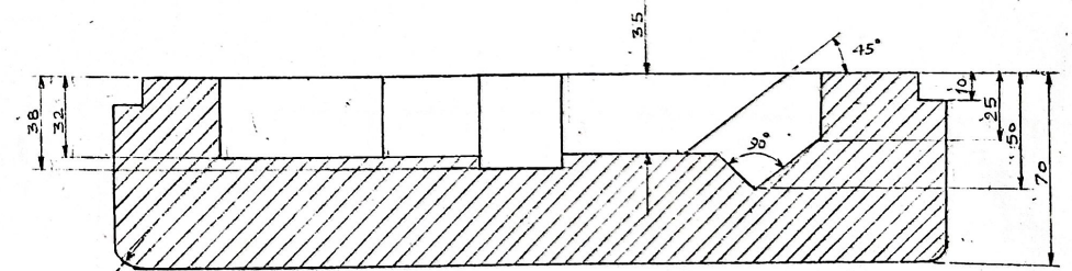
SECTION-BB
