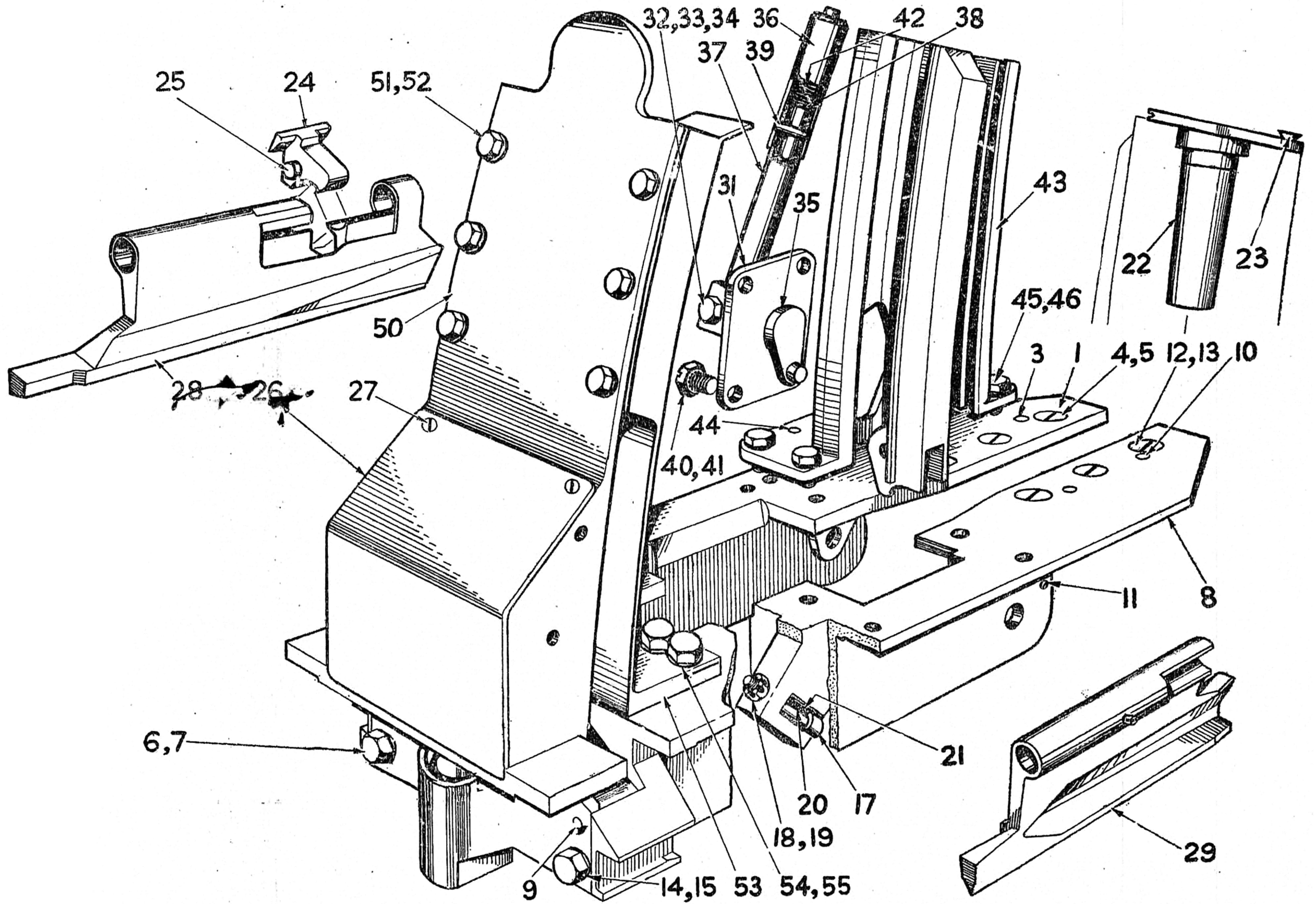
HOOPER ASSY - 1
