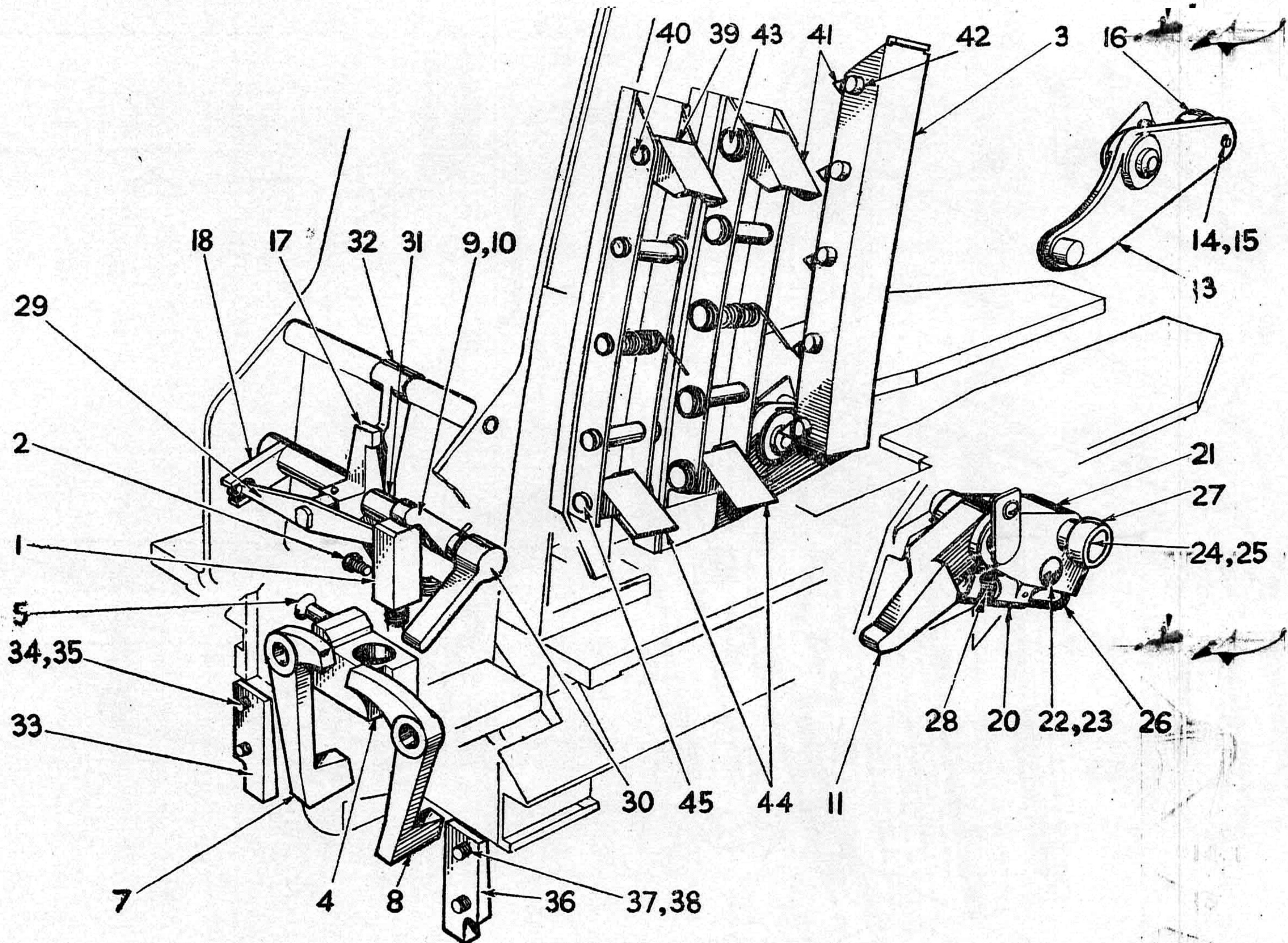
HOOPER ASSY - 2
