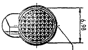
SECTION B-B SCALE 5.000
