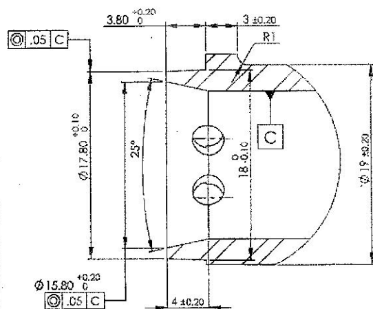
DETAIL N
