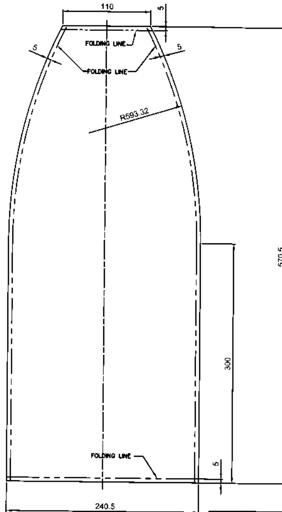
CLOTH COVER (DEVELOPED VIEW)
