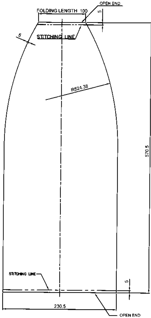
CLOTH COVER FOR SHELL 155MM (ASSEMBLY)
