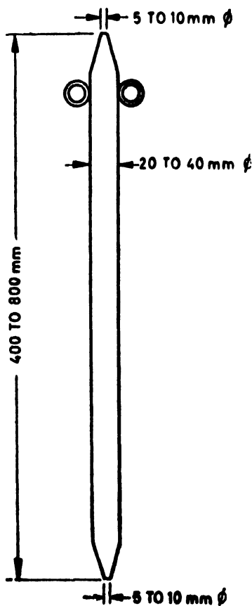
FIG. 7 SAMPLING TUBE
