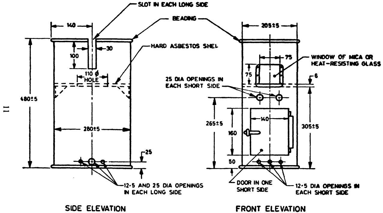
FIG. 2 DRAUGHT SCREEN
