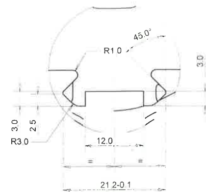
DETAIL X SCALE 2:1
