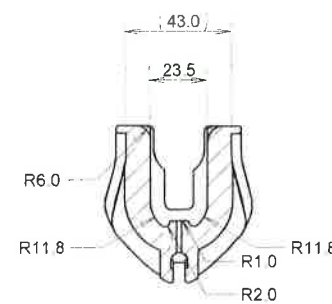
SECTION I-I
