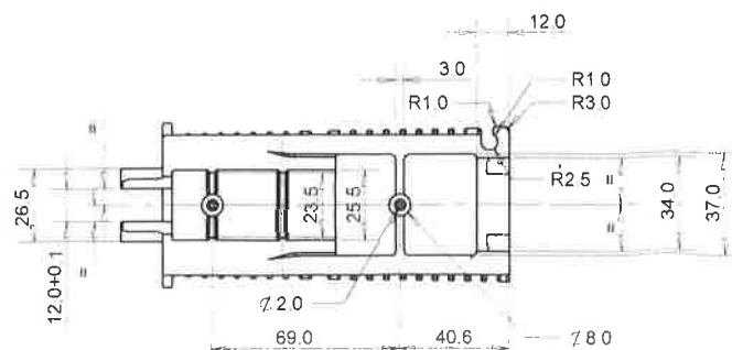
SECTION H-H
