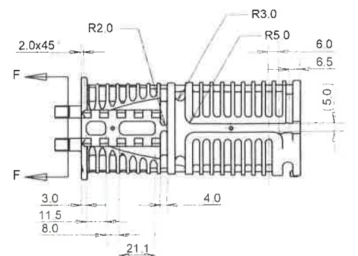
SECTION C-C
