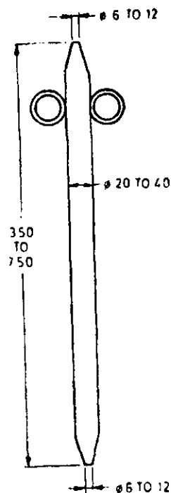
FIG. 3 SAMPLING INSTRUMENT
