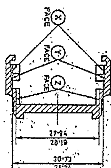
SECTION - 'JJ'
