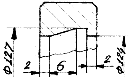
DETAIL OUT OF 'A' SCALE-2:1
